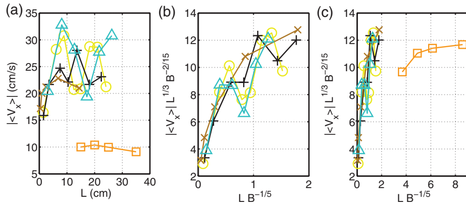
FIG. 15. Rescaling of experimental speed data by factors of length and bending rigidity which correspond to the asymptotic scalings given in Eq. (69). The plot symbols correspond to the foil used (see Table I). Foil A: open triangles (blue), Foil B: open circles (yellow), Foil C: plus signs (black), Foil D: crosses (tan), and Foil E: open squares (orange).
