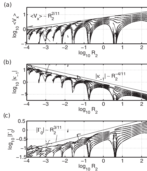
FIG. 12. Results of time-harmonic foil simulations with fixed geometry and eight values of A/L ranging from 0.045 to 0.22: \log_{10} A/L = -1.35, -1.25, -1.15, -1.05, -0.95, -0.85, -0.75, -0.65 . (a) Average swimming speed versus R_2 . (b) Amplitude of leading-edge curvature versus R_2 . (c) Amplitude of circulation versus R_2 .
