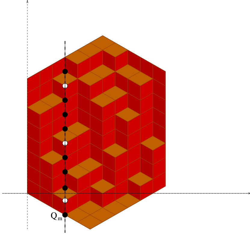
Figure 5: A rhombus tiling of the abc -hexagon, and the lattice \mathcal{L}_m when m = 3 ; holes are represented by white dots and particles are represented by black dots.
