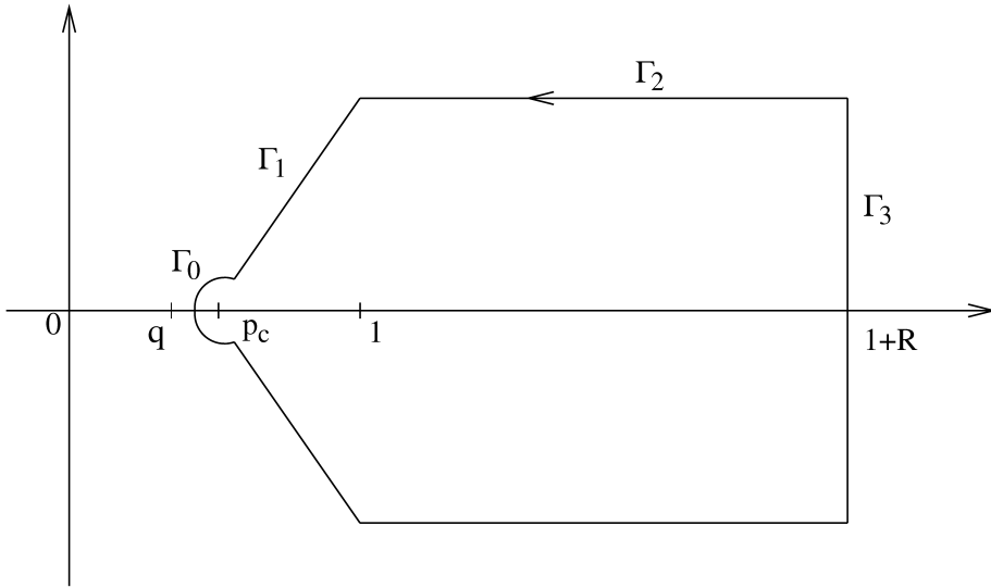
FIG. 4. Contour \Gamma .
