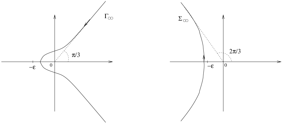
FIG. 3. Contours \Gamma_\infty and \Sigma_\infty of \mathcal{H}(u) and \mathcal{J}(v) .
