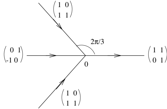
FIGURE 13. \Sigma'' and v_\Psi
