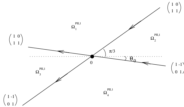
FIGURE 4. p = -q = 1, r = 0 case ; \Sigma_{\theta_0}^{PII,1} and v^{PII,1}
