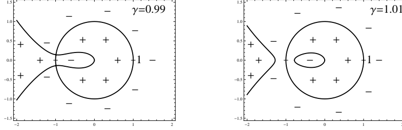
Figure 5. The sign of \text{Re}\theta(z; \gamma) for values of \gamma near \gamma_{\text{crit}} = 1 . Note the sign change near z = -1 on either side of the transition.
