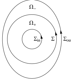
Figure 3. The contours and regions used to define the map \mathbf{Y} \mapsto \mathbf{Q} . The contours \Sigma_{in} and \Sigma_{out} can be deformed as necessary provided they do not intersect \Sigma .
