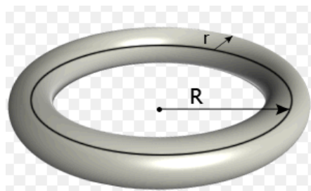
Figure 3.1: 2-torus
