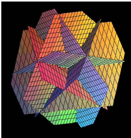
Hyperplane arrangement Type A_3
