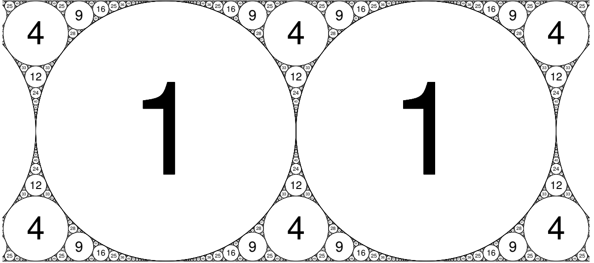
Figure 2: The Apollonian circle packing (0, 0, 1, 1) .
