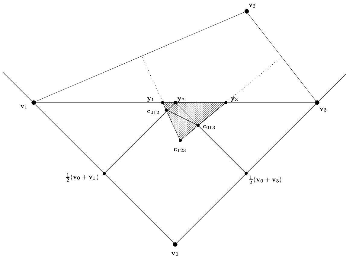
Figure 1: “Tip” of D -simplex [v_1, v_2, v_3]
