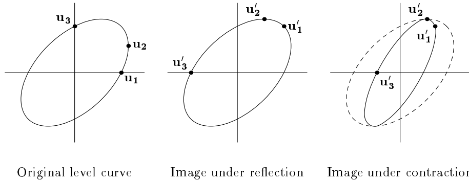
Figure 5: The effects of reflection and contraction moves in \mathbf{u} -space on a level curve of constant Q .
