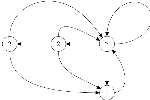
Figure 3: Directed graph depicting legal Nelder-Mead moves for \rho = 1 , \chi = 2 , and \frac{1}{14} \leq \gamma < \frac{1}{8} .
