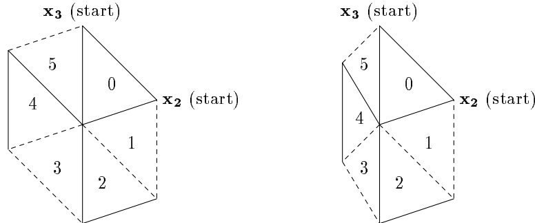
Figure 6: Returning to the original worst point with Nelder-Mead type patterns (1, 1, 1, 1, 1) and (1, 1, \frac{1}{2}, 1, 1) .
