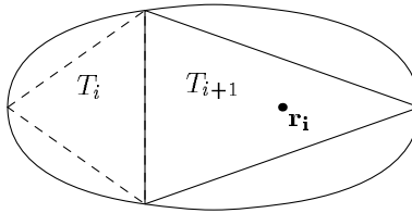
Figure 7: Position of the reflection point \mathbf{r}_i when the vertices of T_i and the expansion point (the new vertex of T_{i+1} ) lie on the boundary of a bounded strictly convex set.
