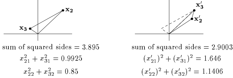
Figure 4: A triangle and its outside contraction.
