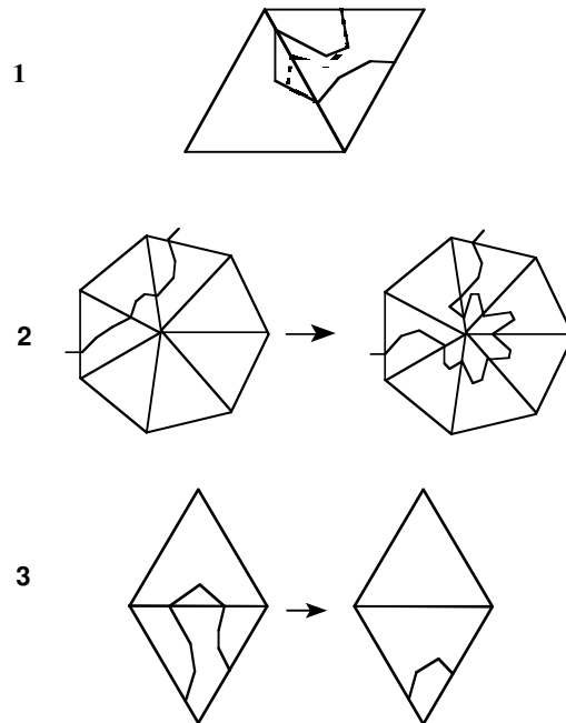
Figure 11: Basic move of types 1, 2 and 3.
