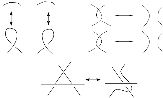
Figure 13: Reidemeister moves of types 1, 2 and 3.
