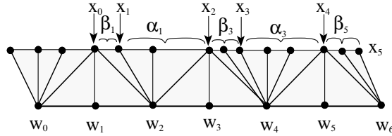
Figure 6: The annulus S_0 .
