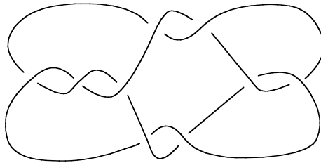
Figure 1: Goeritz's unknot.
