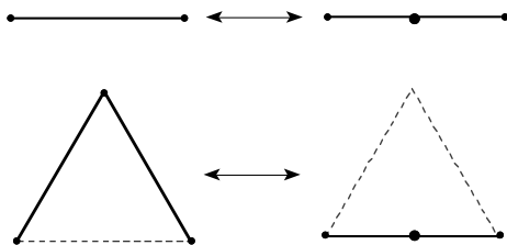
Figure 2: Two types of elementary moves.
