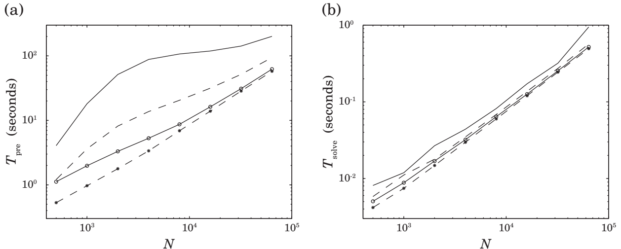
FIG. 5.6. (*) straight channel, (o) converging-diverging channel, (-) serpentine channel, (---) channel with reservoirs. Time in seconds for the precomputation (a) and solve (b) steps versus the number of discretization points N on the walls when the fast direct solver is applied to the geometries in Fig. 5.1.
