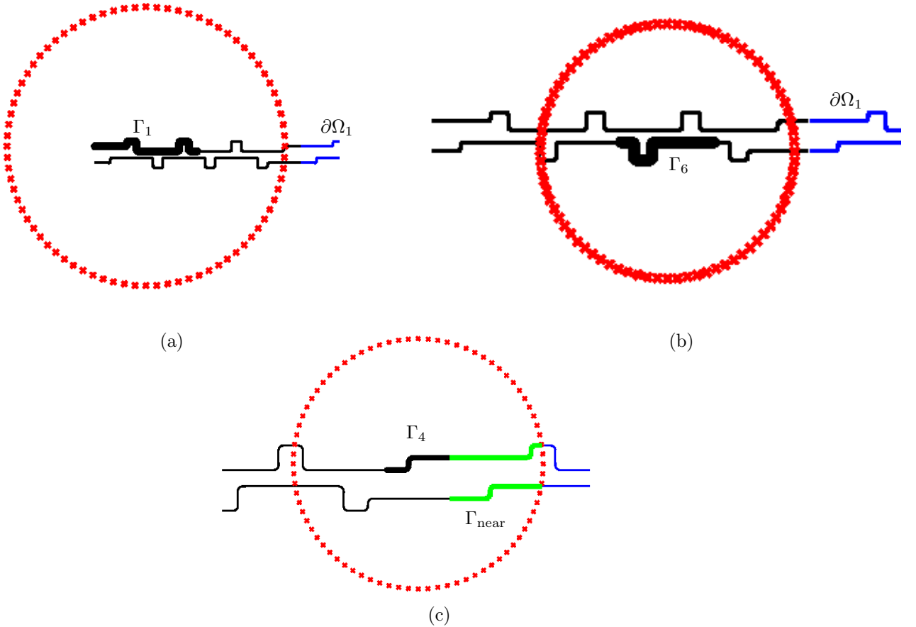
FIG. 4.2. (a) and (b) illustrate the proxy points (red \times symbols) for \Gamma_1 and \Gamma_6 respectively. (c) illustrates the proxy points and the near points \Gamma_{\text{near}} (thick green line) on \partial\Omega_1 for \Gamma_4 . In all figures, \partial\Omega_0 is plotted in black while \partial\Omega_1 is plotted in blue.
