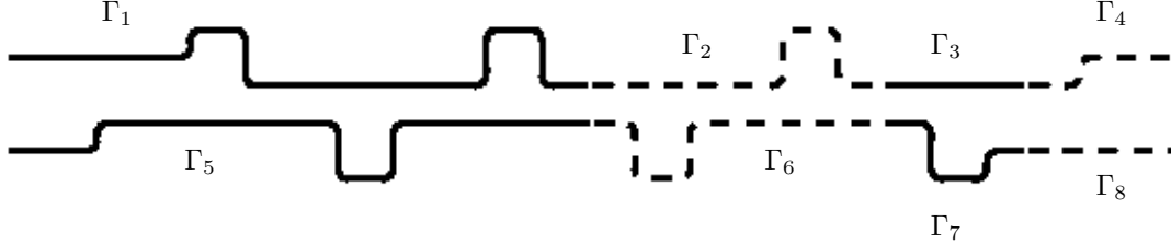
FIG. 4.1. Illustration of the dyadic partitioning of \partial\Omega_0 into Z = 8 sections, used to compress the interaction of the walls in the central unit cell with the right neighbor, i.e. A_1 . Note that the figure shows a single unit cell, for the same channel as in Figure 1.1 and Figure 5.1(d).
